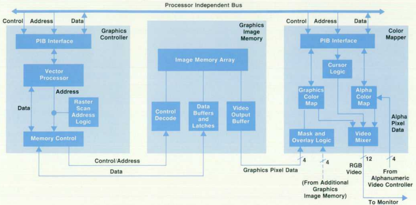
Fig. 2. Graphics hardware modules and functional blocks.
