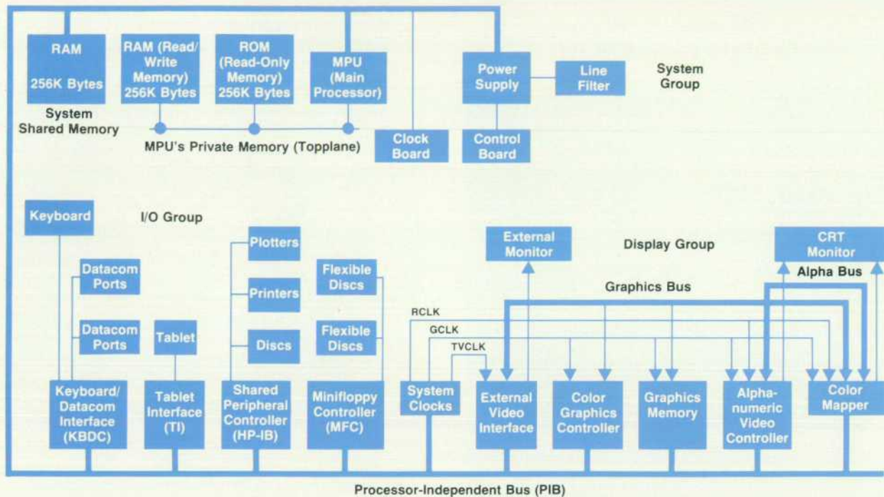
Fig. 2. The HP 2700 has a multiprocessor architecture based on a processor-independent bus. Hardware modules can be divided into three groups.
