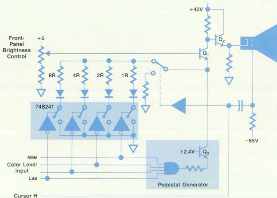
Fig. 1. The video drive circuitry provides 16 color levels to each gun of the CRT and requires four bits of information from the color mapper. This diagram shows the video driver for one color.
