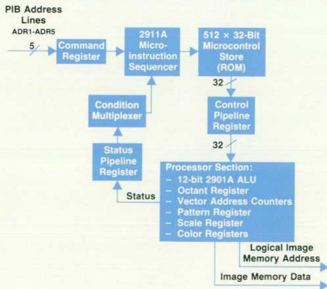
Fig. 3. Vector processor block diagram. Bit-slice hardware from the 2901 family is used.
