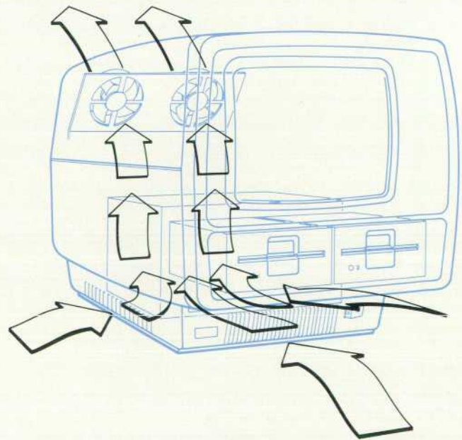
Fig. 1. The HP 2700 has a negative pressure cooling system that uses only two fans.
