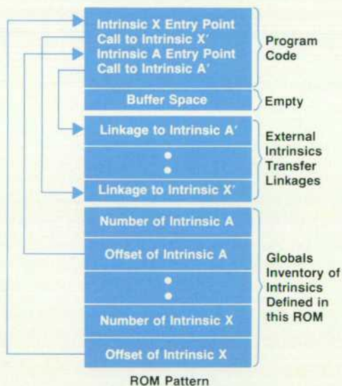
Fig. 1. HP 2700 ROMs are modular and relocatable. Each ROM contains information to link its code to the rest of the maincode.
